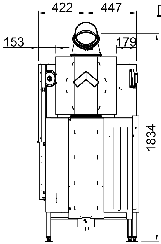
Thermobox, large
